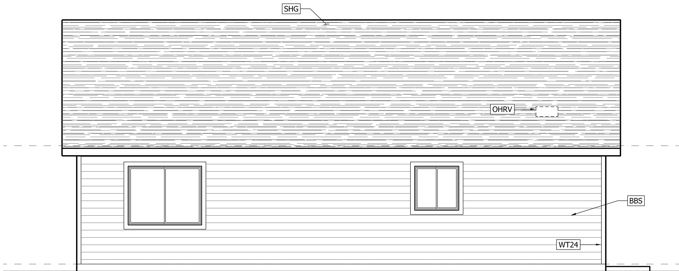
C LEFT ELEVATION 2 1/4" = 1'-0"
