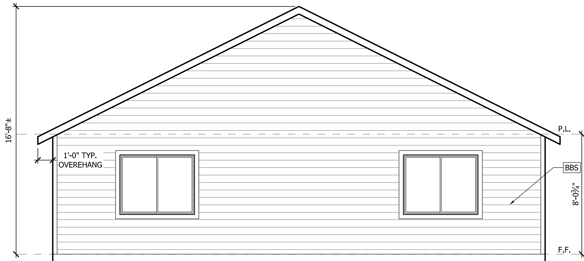
B REAR ELEVATION 2 1/4" = 1'-0"
