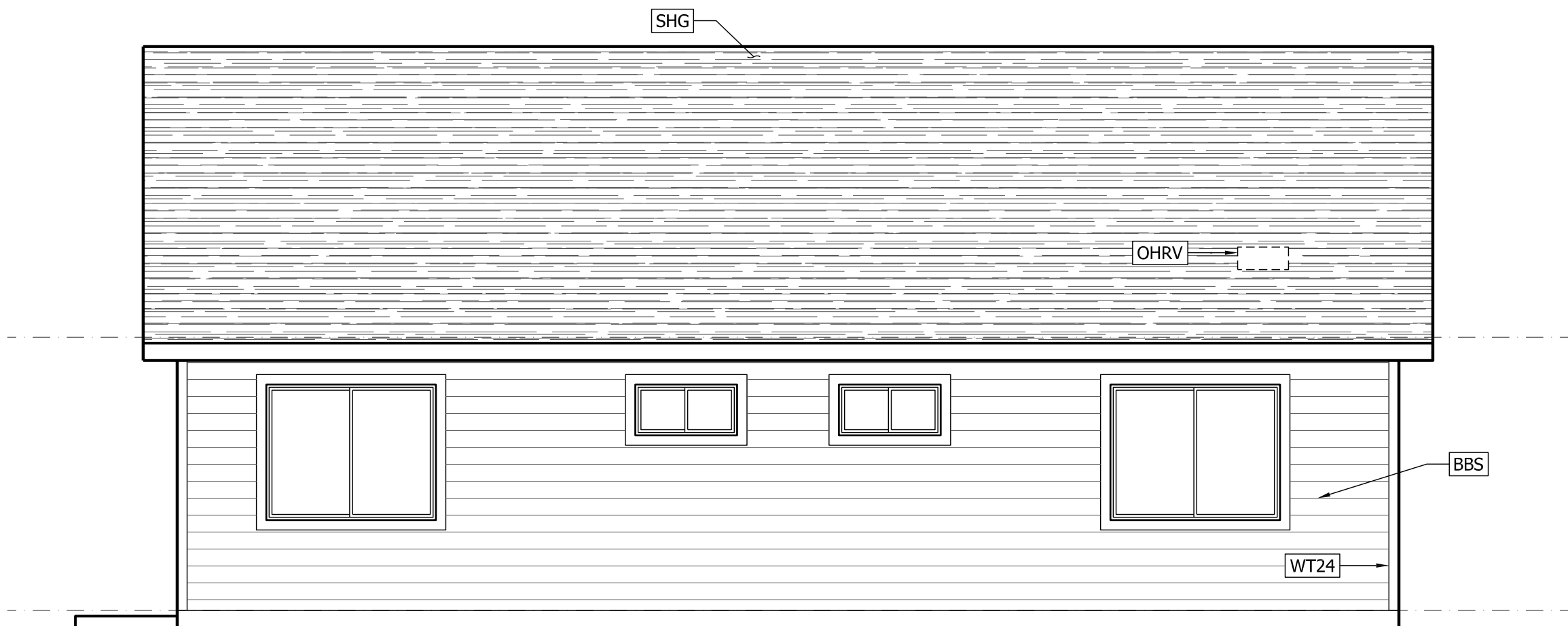
D RIGHT ELEVATION 2 1/4" = 1'-0"
