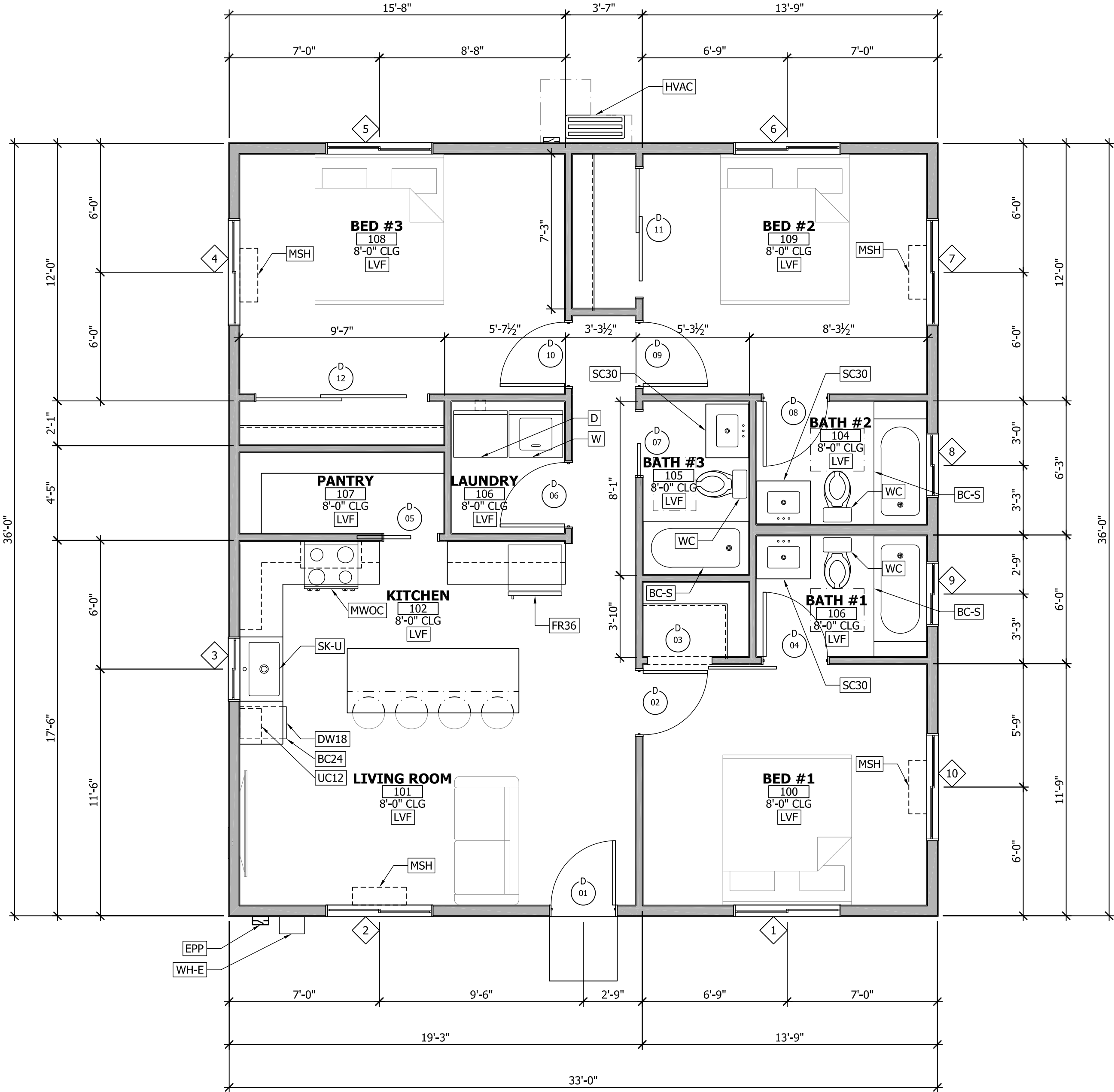
1 FLOOR PLAN
