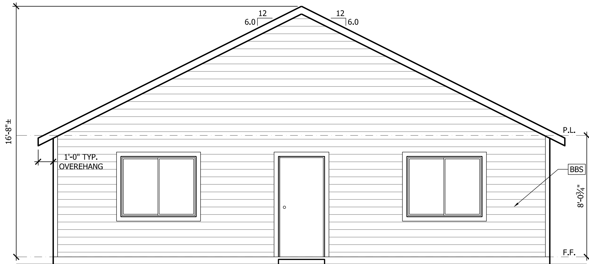
A FRONT ELEVATION 2 1/4" = 1'-0"
